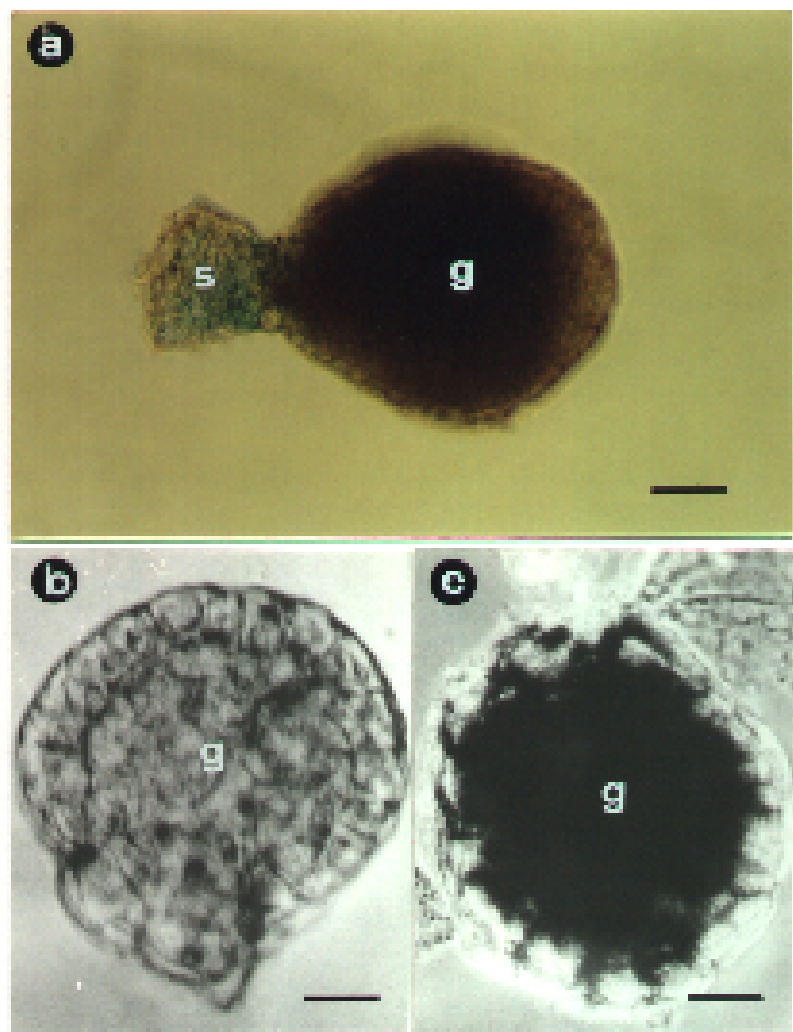
Figure 2. Comparative development of somatic embryos in U. fasciculata . a–b, Globular stage of somatic embryo produced in a seed. Bar in a=0.4 mm. Bar in b=0.35 mm. c, Globular stage of an in vitro-produced somatic embryo. Bar in c=0.35 mm; g=globular embryo; s=suspensor.
