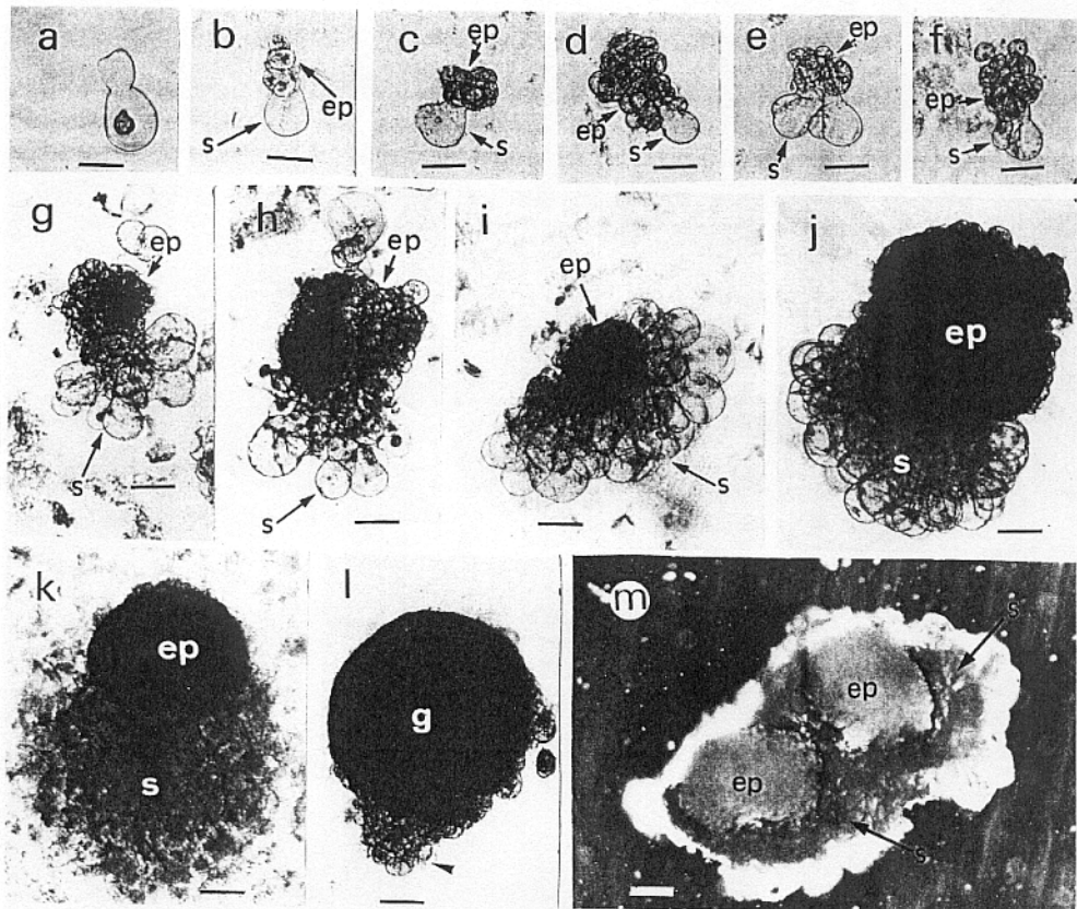
Figure 1. Early development of somatic embryogenesis in Aztekium ritteri . a, First division of the initial embryogenic cell; b-d, First cell divisions of the embryo proper. The avocado-shaped suspensor cell remains single; e, The suspensor cell starts to proliferate; f-k, Different stages of development of the embryo proper and the suspensor; l, Globular somatic embryo; g, with suspensor remains (arrowhead); m, Proembryos showing embryo proper and suspensor. Bars in a through m=0.1 mm; ep=embryo proper, s=suspensor.
